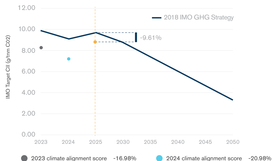
Figure 16. SOCAR Trading climate alignment score, 2018 IMO GHG Strategy 23
